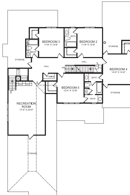
SECOND FLOOR
